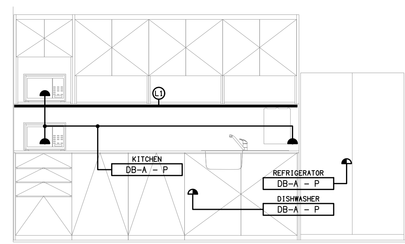
DETAIL B LUNCH ROOM KITCHENETTE SCALE 1:25
